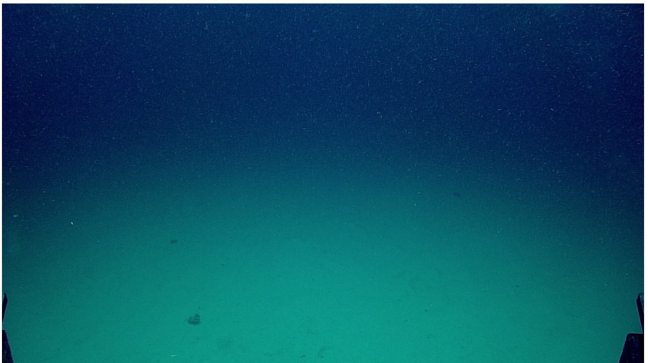
Flat seafloor of the Sohm Abyssal Plain.
